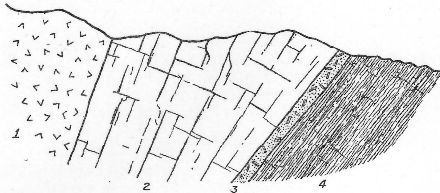
FIG. 9.—Section in pit on lot 3, concession A, Somerville township, Victoria co., Ont.
