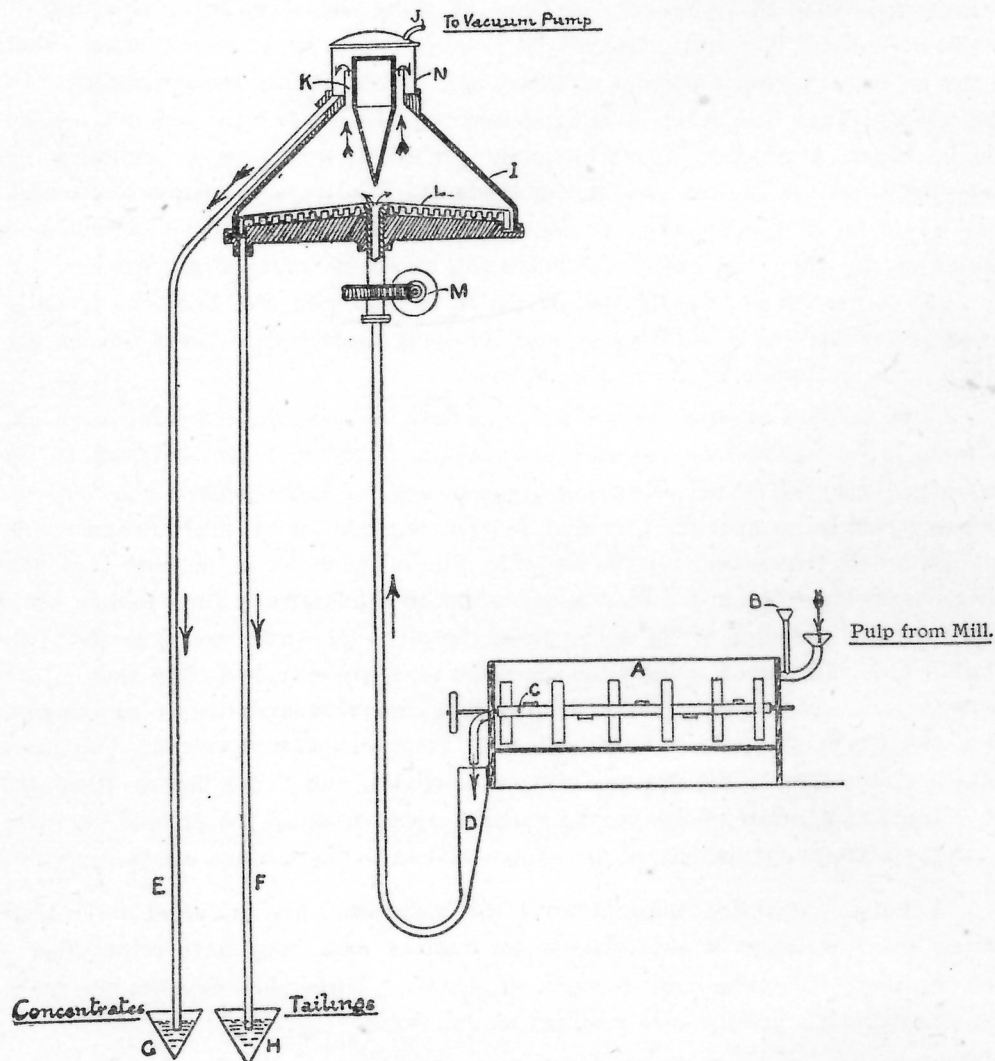
FIG. 2.—Elmore vacuum concentrator: section.
