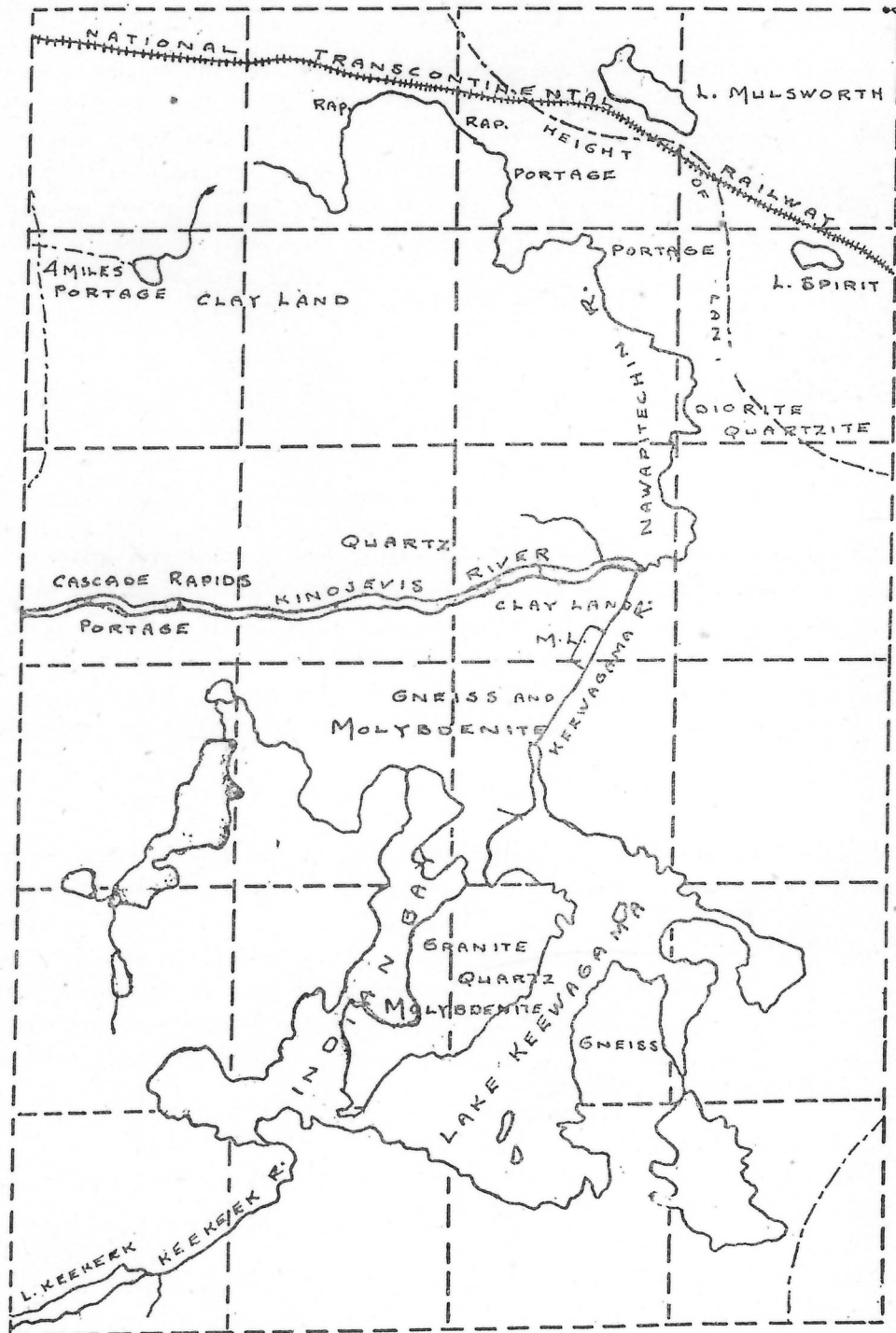
FIG. 8. -Map of the Lake Kewagama molybdenite region, North Pontiac. After Obalski.
