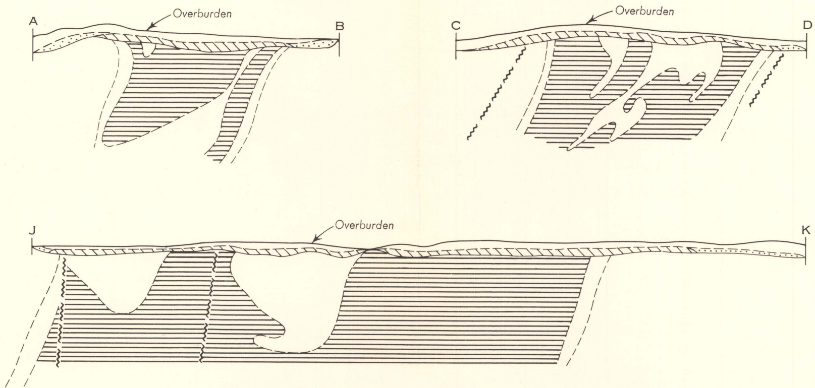
Sections along lines A-B, C-D, and J-K Vertical scale for overburden and gossan enlarged twice
