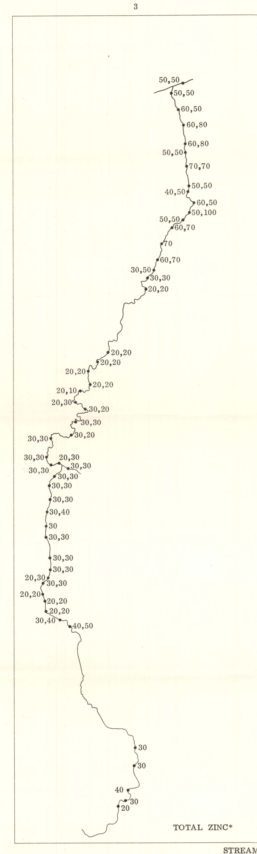
Figure 20. The Geology, aeromagnetics, and stream sediment geochemistry west of North French River, DePencier and Carss Townships, northern Ontario.
