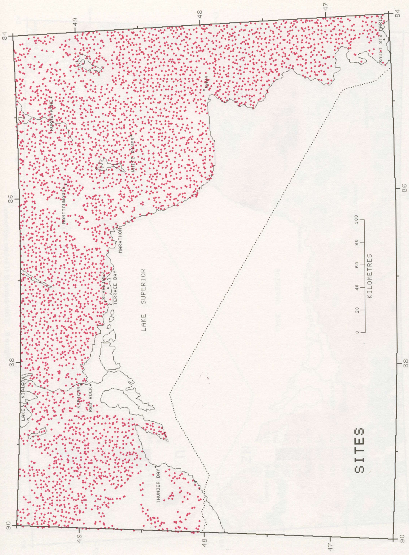
Figure 5. Sample location map.
